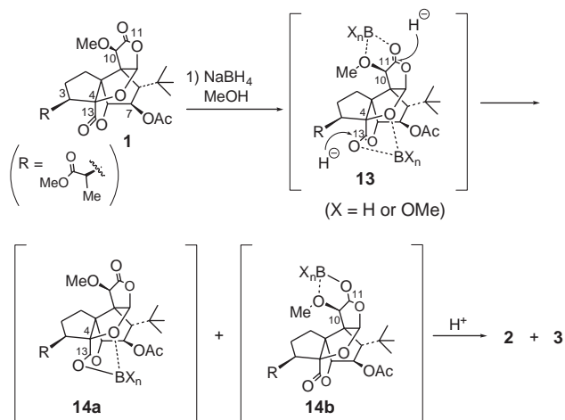
Scheme 3. Possible mechanism of \alpha -alkoxy lactones to lactols.
