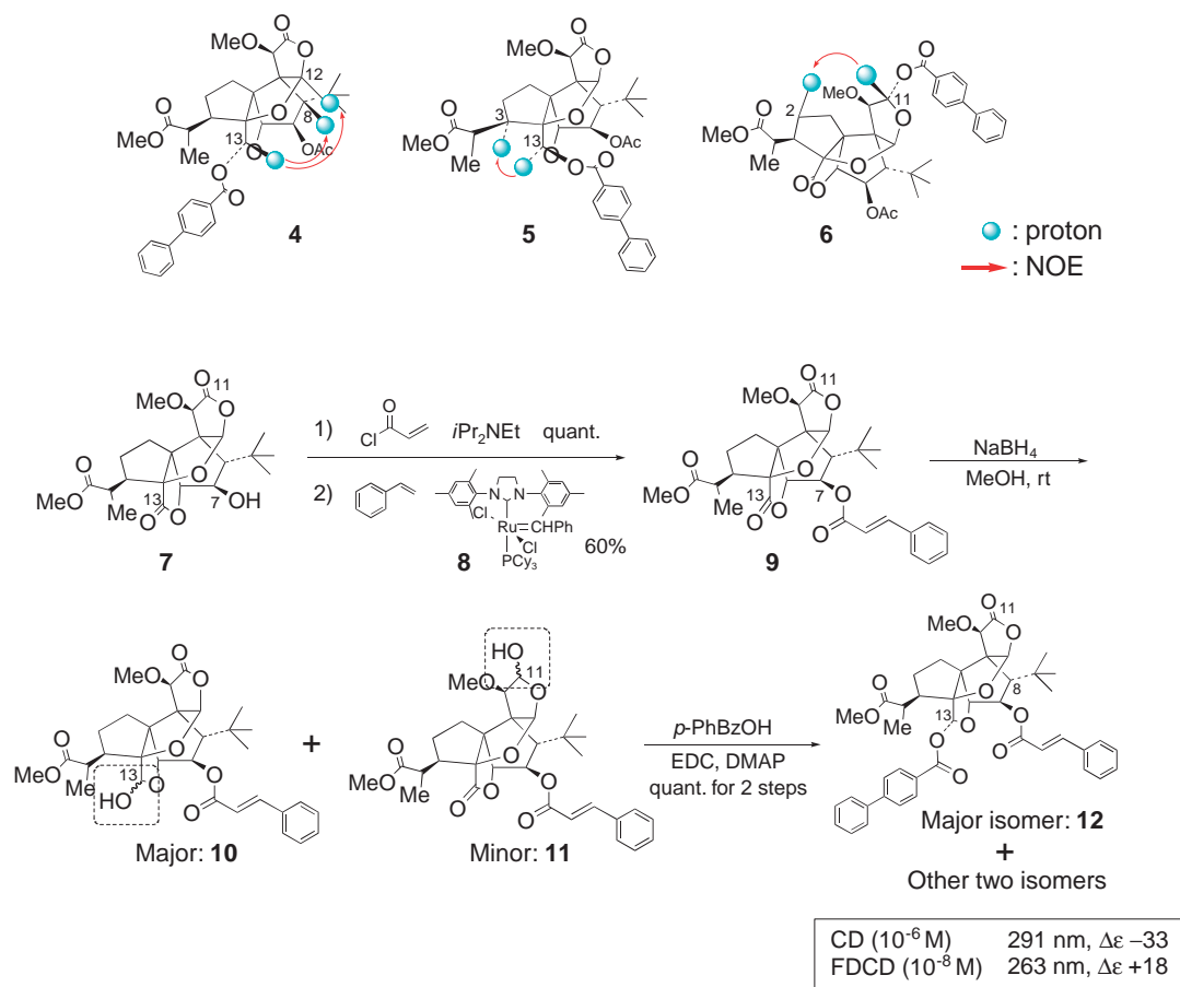
Scheme 2. Stereochemical analysis of reduction products 4-6 and 12 .
