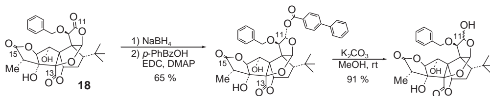
Scheme 4. Synthesis of ginkgolide B lactol derivative.
