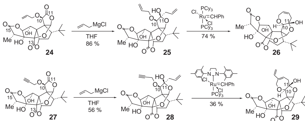
Scheme 6. Preparation of new class of ginkgolide B analogs.
