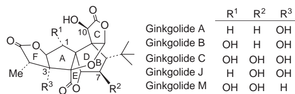
Fig. 1. Structure of five ginkgolides.
