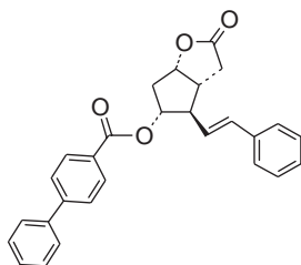
Fig. 2. Structure of Corey lactone.
