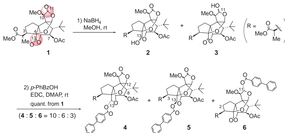
Scheme 1. Reduction of \alpha -alkoxy lactones to lactols.
