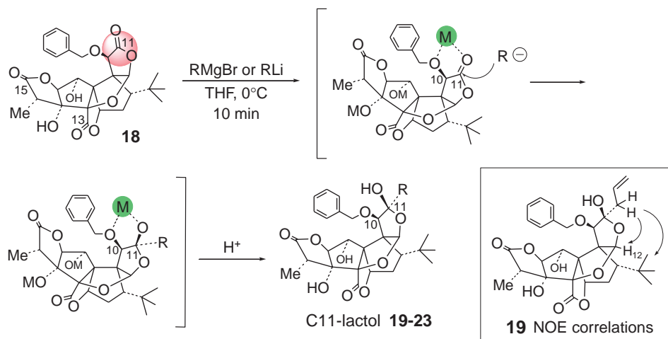
Scheme 4. Synthesis of ginkgolide B lactol derivative.
